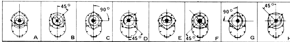
POSITION OF MOUNTING FLANGE-VIEWED FROM FLYWHEEL END
